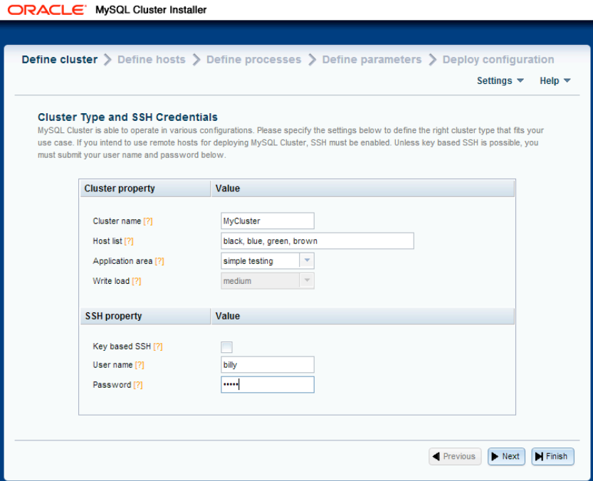
Figure 2. Automated tuning and configuration of MySQL Cluster
