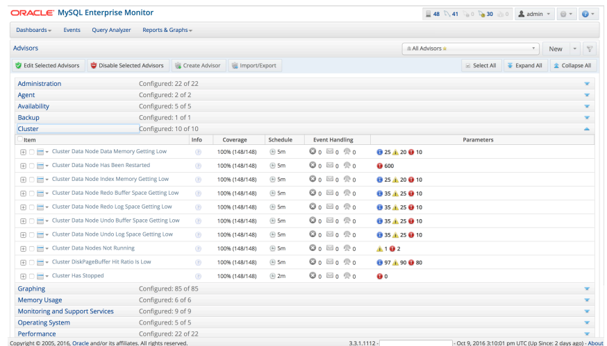
Figure 3. MySQL Cluster expert advisors recommend best practices and reduce the risks of downtime
